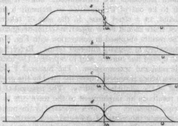
FIG. 8—GRAPHICAL ANALYSIS OF A TRANSMISSION CHARACTERISTIC
