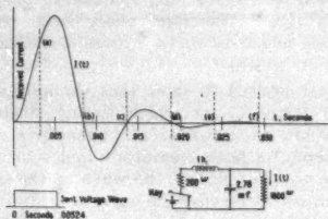
FIG. 5—INSTANCE OF NON-DISTORTING WAVE
