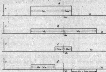
FIG. 7—GRAPHICAL ANALYSIS OF A TRANSMISSION CHARACTERISTIC
