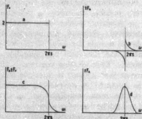
FIG. 2—IDEAL SHAPE FACTORS
