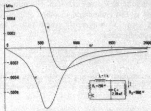
FIG. 6—TRANSFER ADMITTANCE, u + ie , CORRESPONDING TO THE NON-DISTORTING WAVE SHOWN IN FIG. 5
