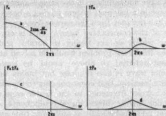
FIG. 3—IDEAL SHAPE FACTORS
